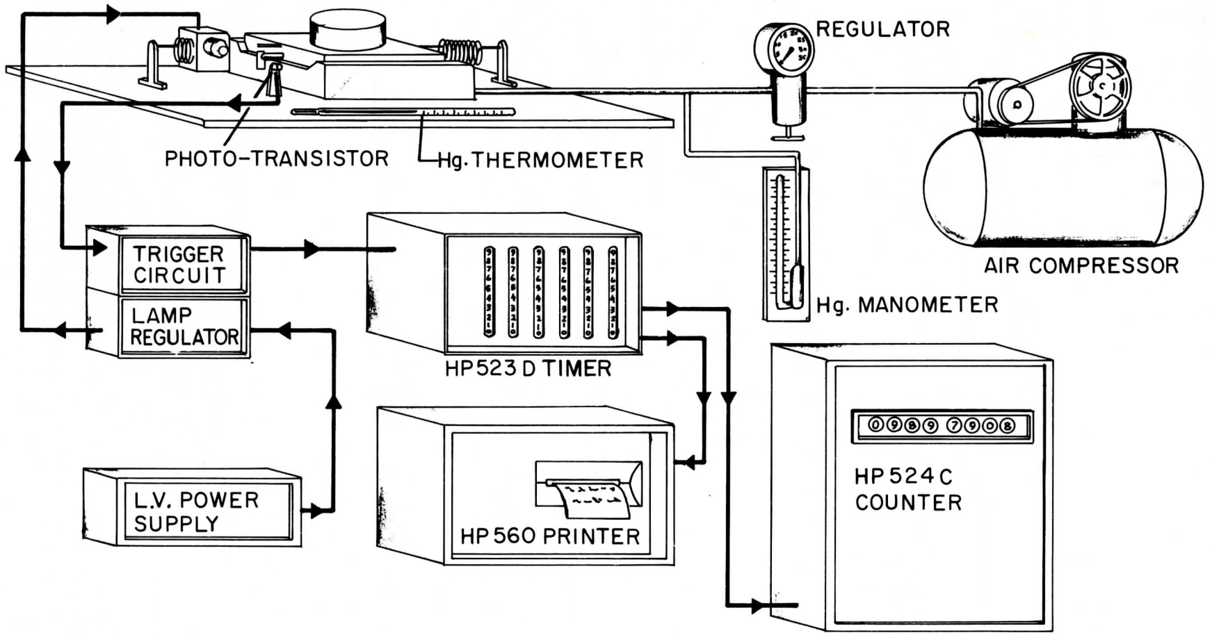
Figure 4.1.4 Instrumentation and Accessory Arrangement of Phase I Pendulum
