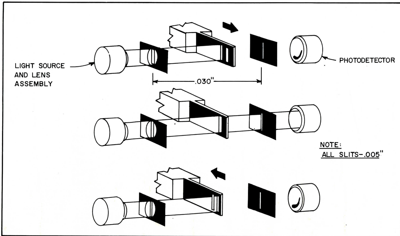
Fig. 5 ZERO CROSSING DETECTOR ARRANGEMENT SHOWING A CROSSING CYCLE
